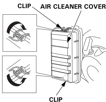
AIR FILTER ELEMENT
