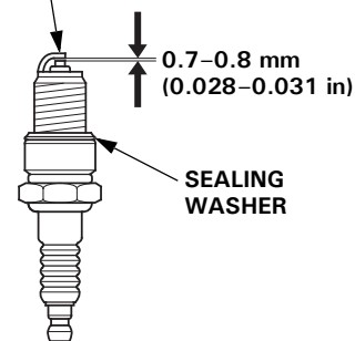
SIDE ELECTRODE
